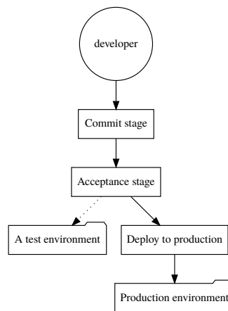
Figure 5.1: The default pipeline
